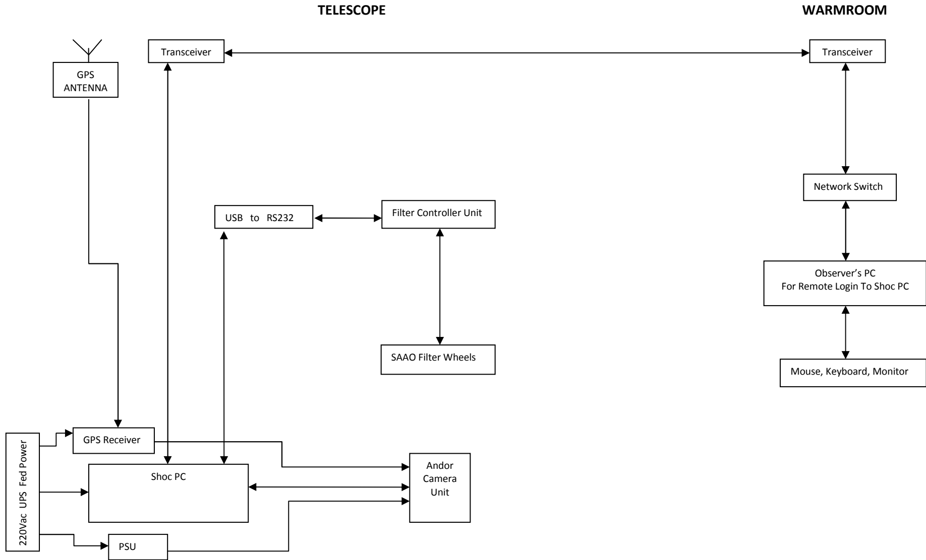
SHOC DIAGRAM – Applicable to 1.9m; 1m & 0.75m Telescopes (as at Feb 2014 - JC)
